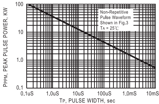
FIG. 1 - PULSE POWER RATING CURVE
